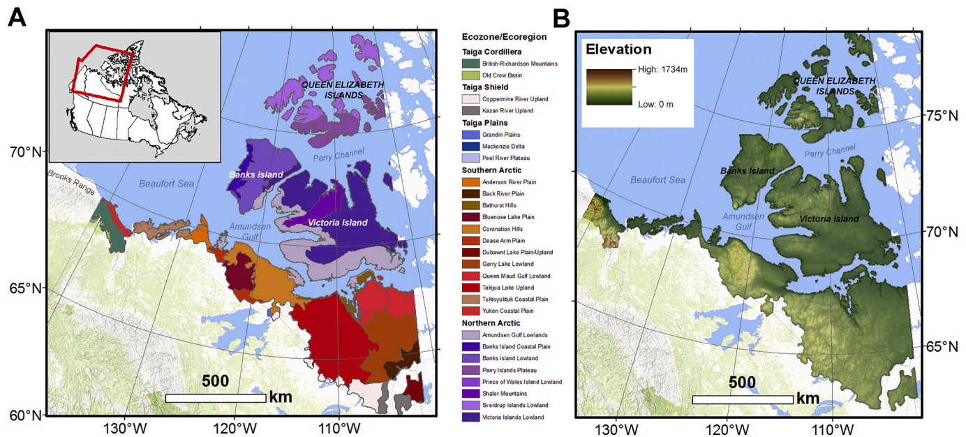
Fig. 1. (A) Map of the study region in the western Canadian Arctic overlaid with colours distinguishing ecoregions and ecozones located in this area. Inset map in upper left shows the extent of the 80-million hectare study area in north-western Canada. (B) Map of the study region overlaid with a Digital Elevation Model.
