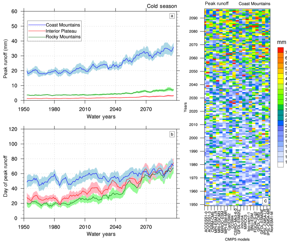
Figure 7. CMIP5-VIC-simulated daily peak runoff (a) and corresponding day of the peak runoff (b) in the cold season of the water year for the Coast Mountains, Interior Plateau and Rocky Mountains. Solid curves are for the MME mean, and shading represents inter-model spread, as represented by a 5 %–95 % model range. A 5-year running mean is applied to smooth variations in all curves; y-axis values in (b) represent days of water year, where 0 corresponds to 1 October. (c) Cold season peak runoff (in mm) simulated by individual CMIP5-VIC simulations for the Coast Mountains.
