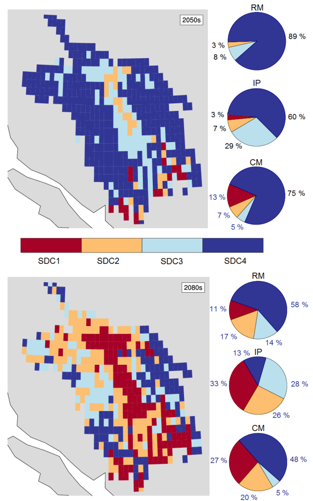
Figure 9. CMIP5-VIC-simulated MME mean projected snowmelt-dominant categories (SDC) in the 2050s and 2080s. SDCs are classified using the SP detection algorithm (described in Sect. 2.5) and are based on changes (%) in the fraction of years with SP. Pie charts show corresponding change in fraction of grid cells (%) in each SDC for the geoclimatic regions of the Rocky Mountains (RM), Interior Plateau (IP) and Coast Mountains (CM).
