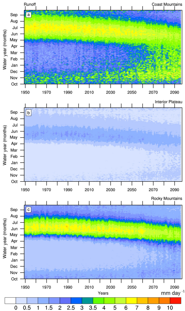
Figure 6. CMIP5-VIC-simulated MME mean daily runoff for the Coast Mountains (a), Interior Plateau (b) and Rocky Mountains (c). Values are spatial averages over geoclimatic regions. Units are \text{mm day}^{-1} . Runoff units are an equivalent regional average rainfall rate rather than a discharge rate.
