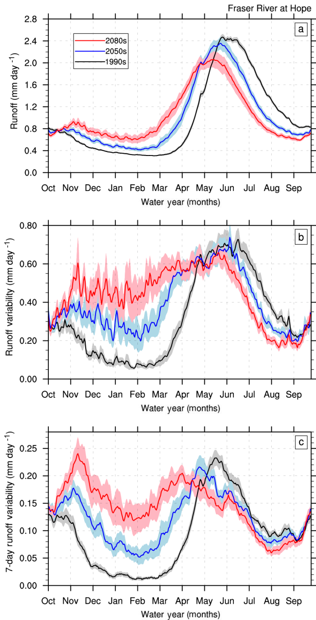
Figure 8. CMIP5-VIC-simulated daily runoff (normalized discharge) mean (a), variability (b) and 7-day variability (c) for the Fraser River at Hope. Black, blue and red curves represent the MME mean for the 1990s, 2050s and 2080s, respectively. Shading represents inter-model spread, as indicated by a 5%–95% model range.
