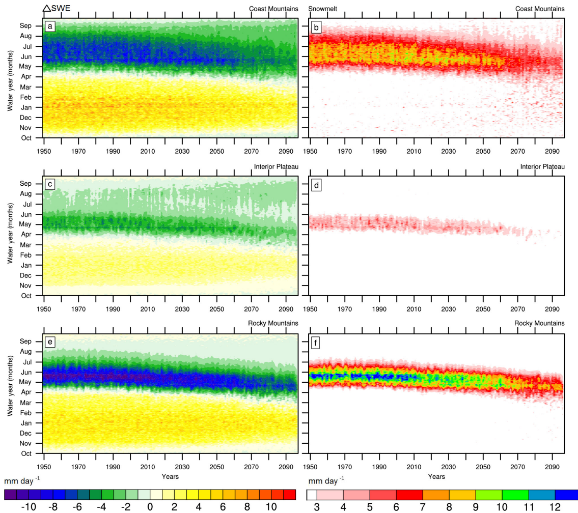
Figure 5. CMIP5-VIC-simulated MME mean \Delta SWE (daily SWE rate) (a, c, e) and snowmelt (b, d, f) for the Coast Mountains (a, b), Interior Plateau (c, d) and Rocky Mountains (e, f). In (a), (c) and (e), values greater than 0 represent snow accumulation, while those below 0 indicate snow ablation. Units are \text{mm day}^{-1} .
