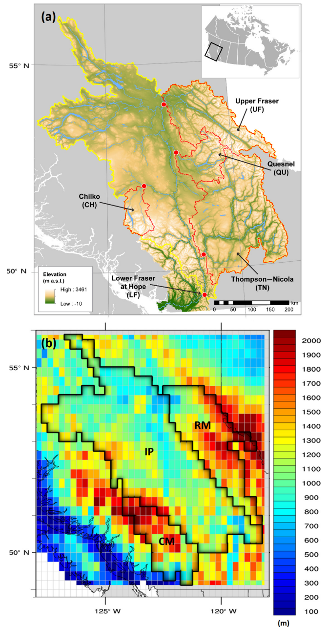
Figure 1. (a) Digital elevation model of the FRB with identification of sub-basins: upper Fraser (UF), Quesnel (QU), Chilko (CH), Thompson–Nicola (TN) and Fraser at Hope (LF). (b) Elevation map highlighting the Fraser River Basin and three geoclimatic regions. RM, IP and CM represent the Rocky Mountains, Interior Plateau and Coast Mountains, respectively. Elevations are in metres, and the horizontal grid resolution is that of the VIC hydrological model (0.25°).
