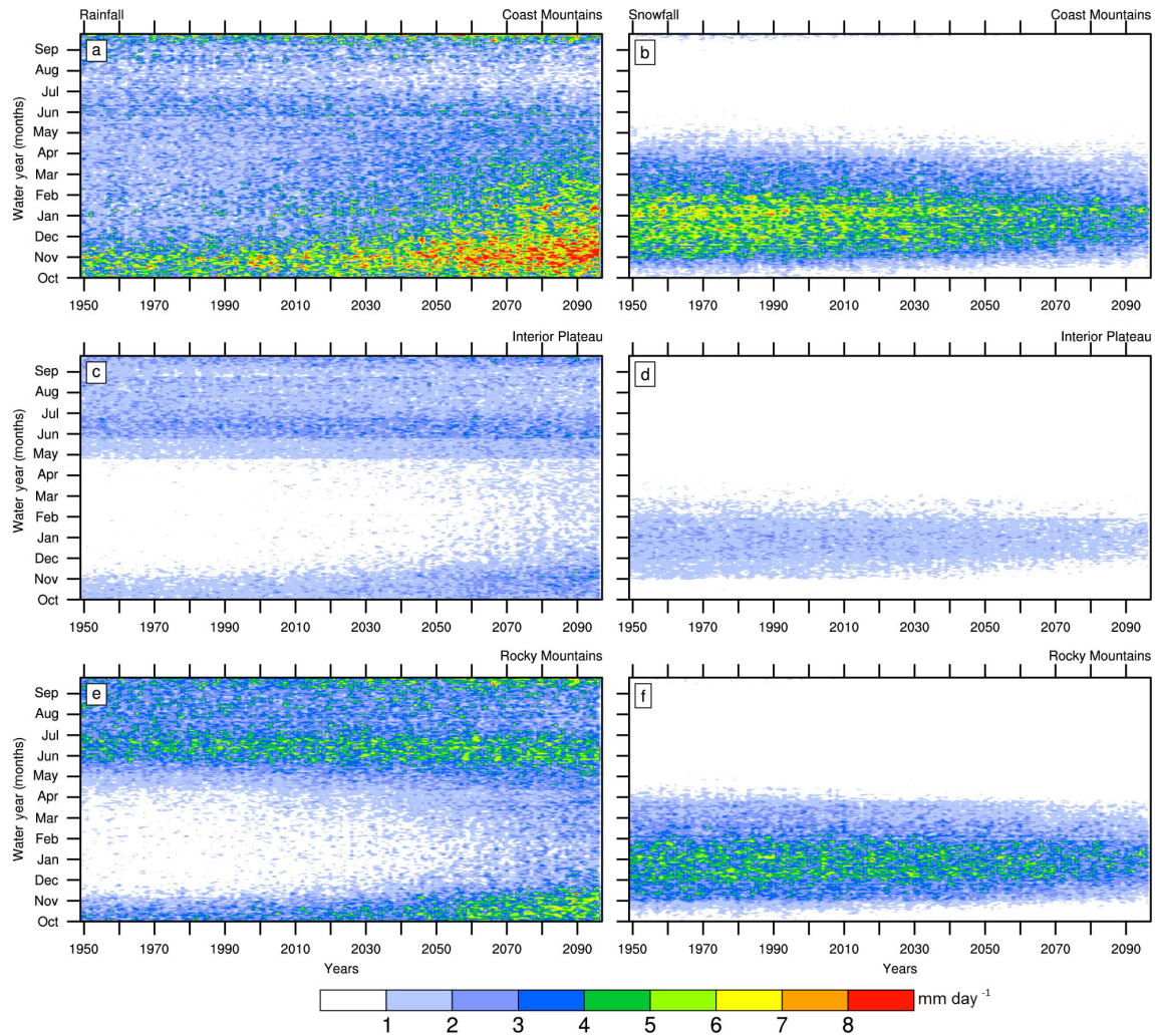
Figure 4. Partitioning of CMIP5 MME mean total precipitation into daily rainfall (a, c, e) and snowfall (b, d, f) for the Coast Mountains (a, b), Interior Plateau (c, d) and Rocky Mountains (e, f). Values are regional spatial averages over the three geoclimatic regions. Units are \text{mm day}^{-1} .
