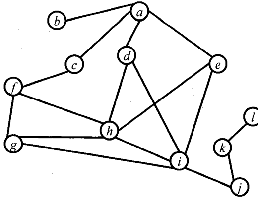
Figure A2. An illustration of a connected graph.
