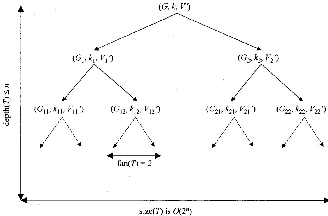
Figure 2.3. Illustration of the Exhaustive Vertex Cover algorithm.
