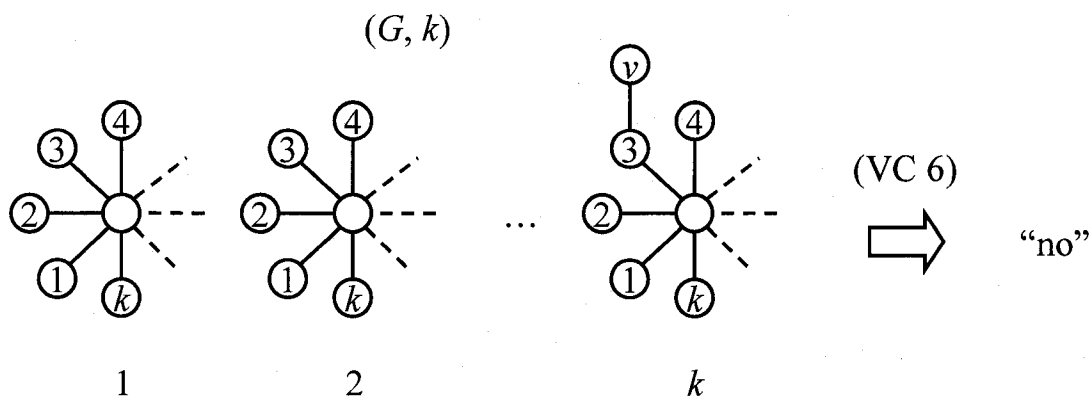
Figure 4.2. Illustration of rule (VC 6) and the intuition behind its proof.
