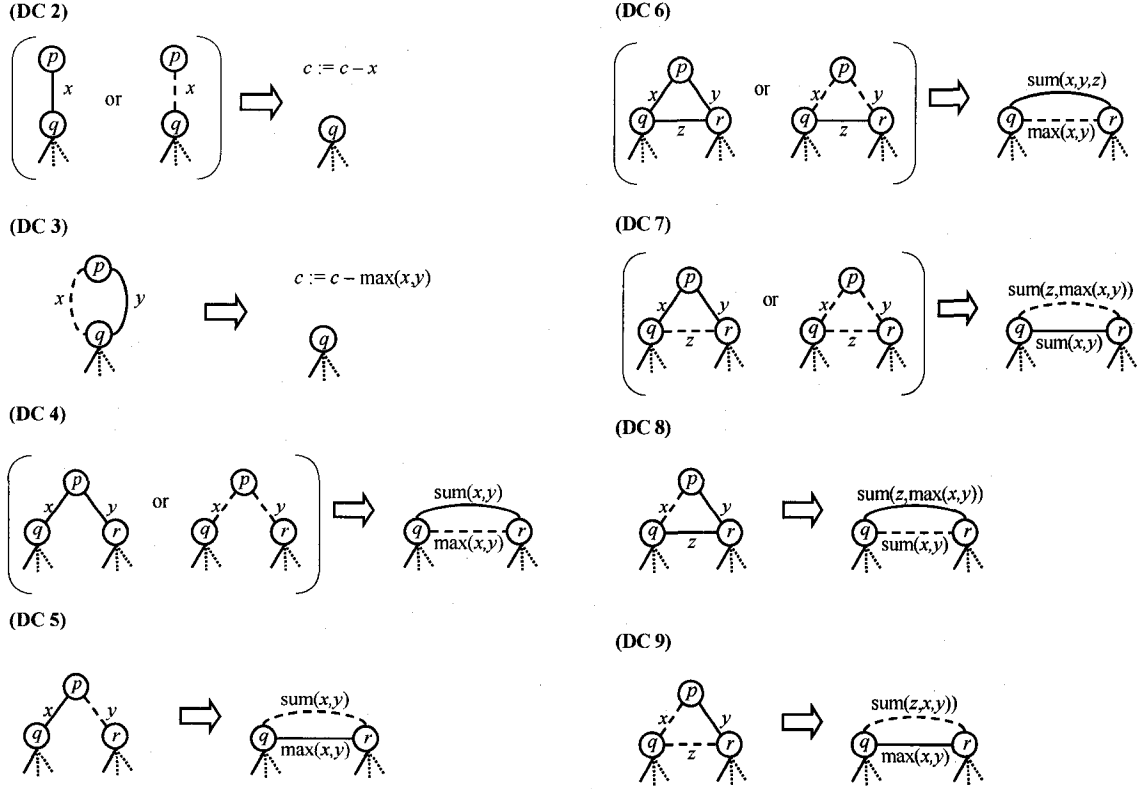
Figure 5.2. Illustration of the reduction rules for Double-Constraint Coherence. Reduction rules (DC 2)–(DC 9) are illustrated. Solid lines represent positive constraints and dotted lines represented negative constraints. The symbols x , y and z represent weights. See text for details.
