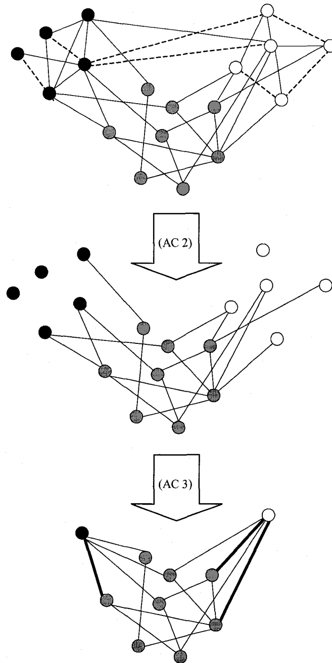
Figure 5.3. Illustration of reduction rules (AC 2) and (AC 3). Here the rules (AC 2) and (AC 3) are applied to an instance for a Pos-Annotated Coherence. Positive constraints are indicated by solid lines and negative constraints by dotted lines. The black dots represent elements in A' , the white dots represent elements in R' , and the gray dots represent elements in P' . Application of (AC 2) to the instance results in the removal of all constraints with both endpoints in A' \cup R' , and subsequent application of (AC 3) results in merging all elements in A' into one element s , and in merging all elements in R' into one element t . The bold lines in the bottom figure indicate that the weights of those constraints have been changed in the merge procedure of (AC 3). Note that the instance at the bottom is an instance for the Min-Cut problem.
