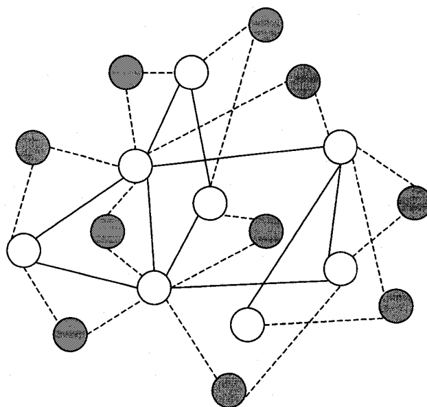
Figure 3.2. Illustration of the reduction in Lemma 3.1.
