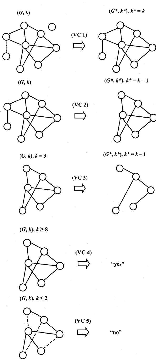
Figure 4.1. Illustration of reduction rules (VC 1) – (VC 5) for Vertex Cover.
