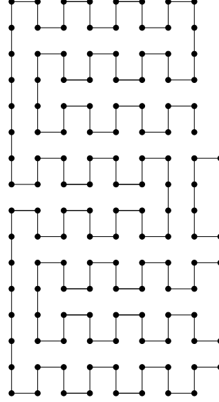
FIGURE 2. A wiggly lattice path
