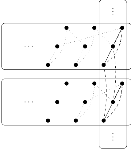
FIGURE 1. Cycle merging illustration
