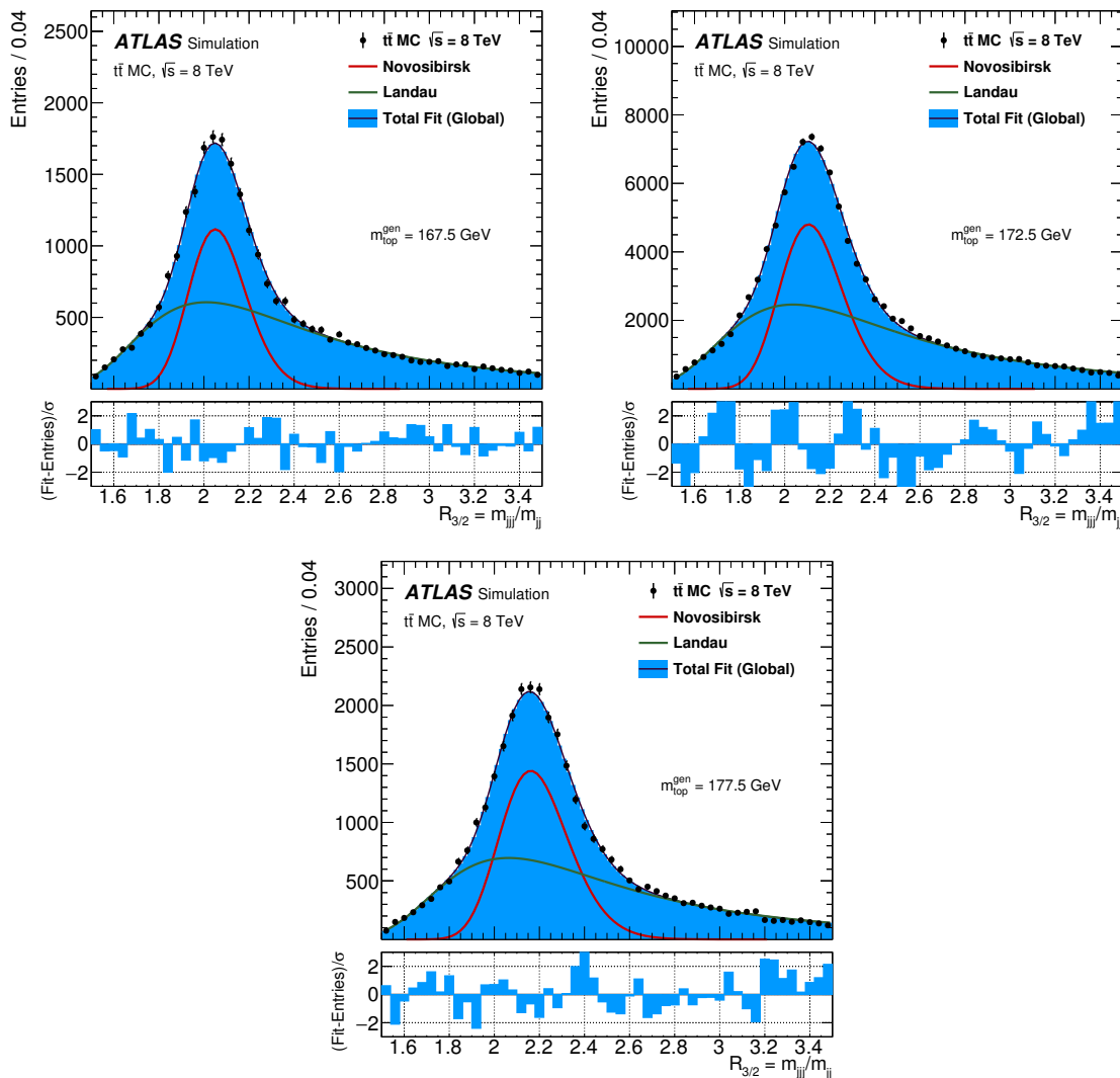
Figure 3. Templates for the R_{3/2} distributions for t\bar{t} MC samples generated at m_{top} values of 167.5, 172.5, and 177.5 GeV, respectively. Results from the combined, simultaneous fit to all five R_{3/2} distributions are superimposed (black line with blue filled area). For each distribution it consists of a Novosibirsk function (red line) describing the signal part and a Landau function (green dashed-line) describing the combinatorial background part. Their parameters are assumed to depend linearly on m_{top} . The \chi^2 per degree of freedom obtained for each of the three template distribution corresponds to 1.22, 3.98, and 1.96 respectively. The plot under each distribution shows the residuals obtained from calculating the difference between the combined fit and the simulated R_{3/2} distribution normalised to the statistical uncertainty for each bin individually.
