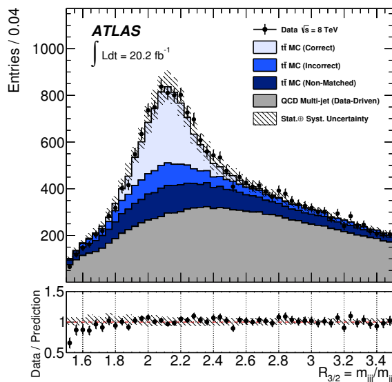
Figure 2. R_{3/2} distribution as obtained after applying the analysis event selection shown together with the expected sum of t\bar{t} simulation and multi-jet background. The distribution is shown before the \chi^2 fit is applied. The ratio comparing data to prediction is shown below the figure. The hatched bands reflect the sum of the statistical and systematic errors added in quadrature. The t\bar{t} simulation corresponds to m_{\text{top}} = 172.5 GeV.
