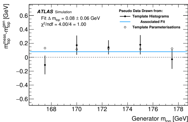
Figure 5. The difference mean, (m_{top}^{meas} - m_{top}^{gen}) , based on the results of a fit to a single Gaussian function. The black markers correspond to cases where the pseudo events were drawn from the R_{3/2} histograms, and the open marker points where pseudo events were drawn from the parameterisations. The solid blue line corresponds to a polynomial fit to the five black markers and their corrected uncertainties.
