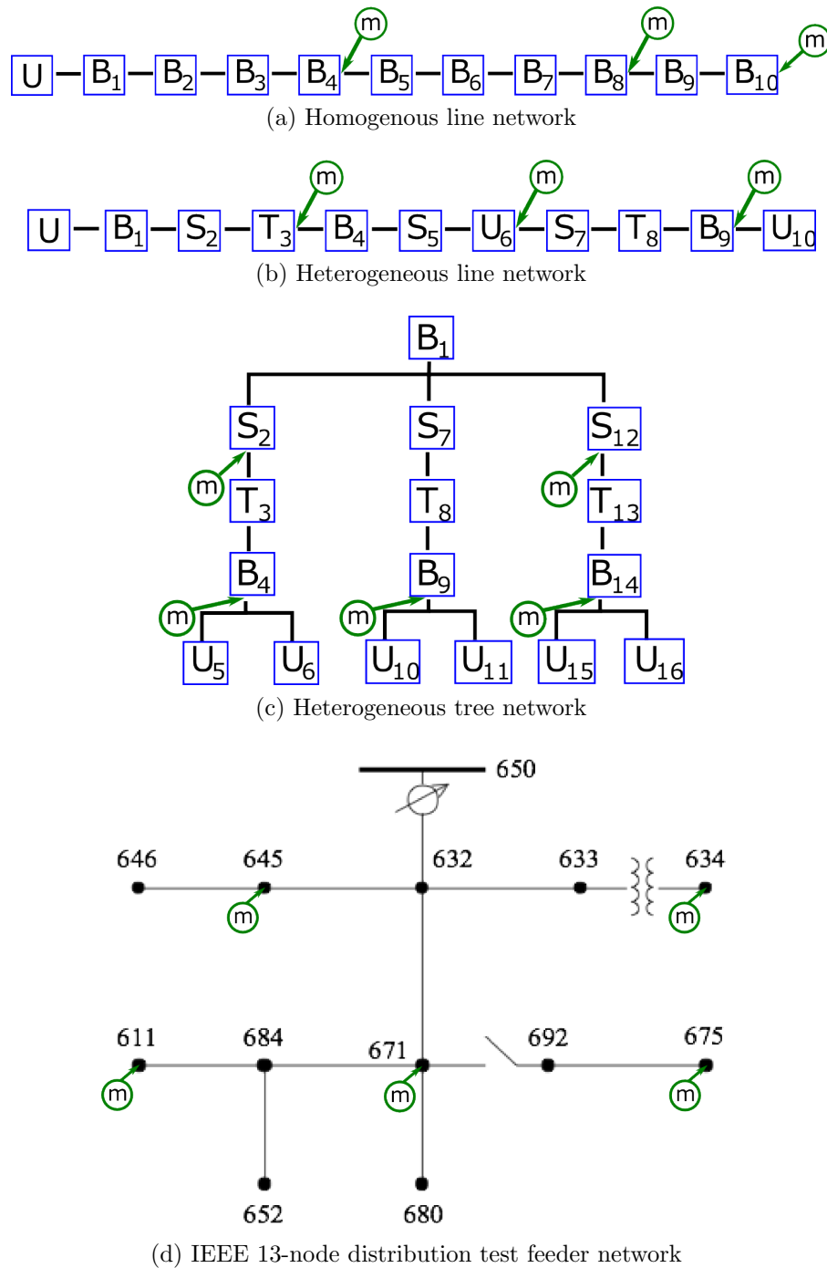
Figure 7.5: Networks used in our experiments. B=bus, S=switch, T=transformer, U=UPS. The circled m indicates the position of a meter. The meter positions are based on our meter placement solution proposed in Chapter 5.
