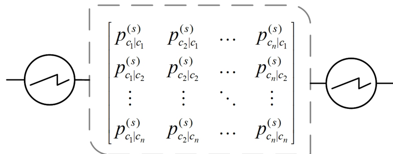
(b) Subnet as a single power transition matrix.
