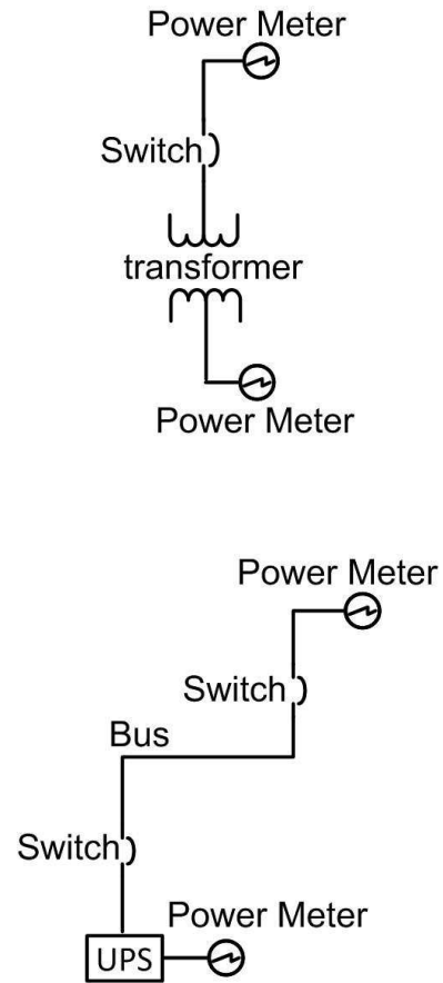
Figure 6.3: Two different kinds of subnets. The one at the left side containing two devices (switch, transformer) and the one shown at the right side containing four devices (switch, bus, switch, and UPS).
