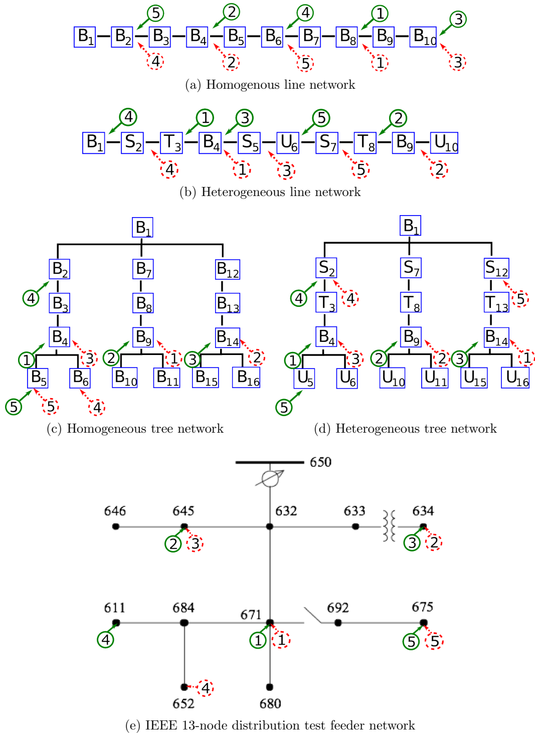
Figure 5.4: Networks used in our experiments. B=bus, S=switch, T=transformer, U=UPS. Ordered dotted circles correspond with the sequence of meters placed by BP while the solid circles show the meter placed by MinEntropy.
