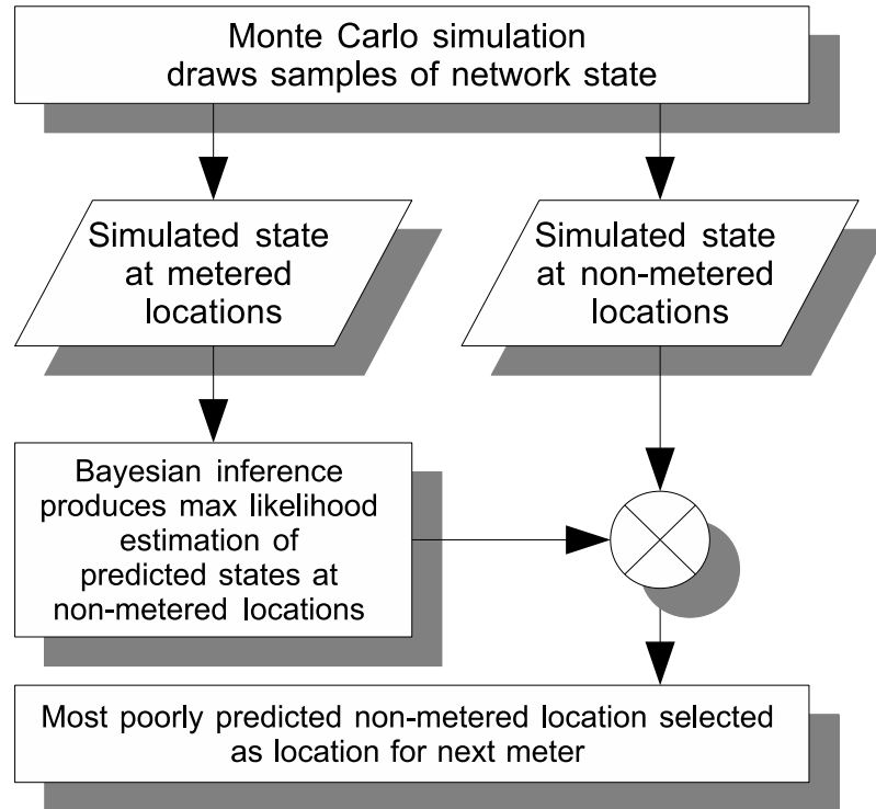
Figure 5.1: Data flow diagram of meter selection process during a single iteration of the greedy algorithm.
