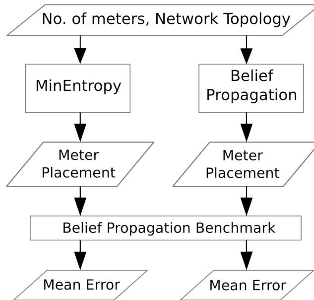
Figure 5.3: An overview of the meter placement evaluation process.
