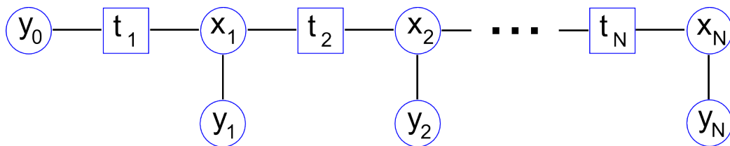
Figure 5.2: Power network modeled as a factor graph
