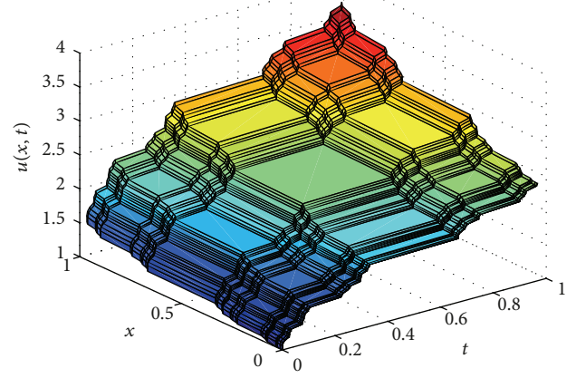
FIGURE 2: Plot of u(x, t) with the parameters \alpha = \ln 2 / \ln 3 and k = 50 .
