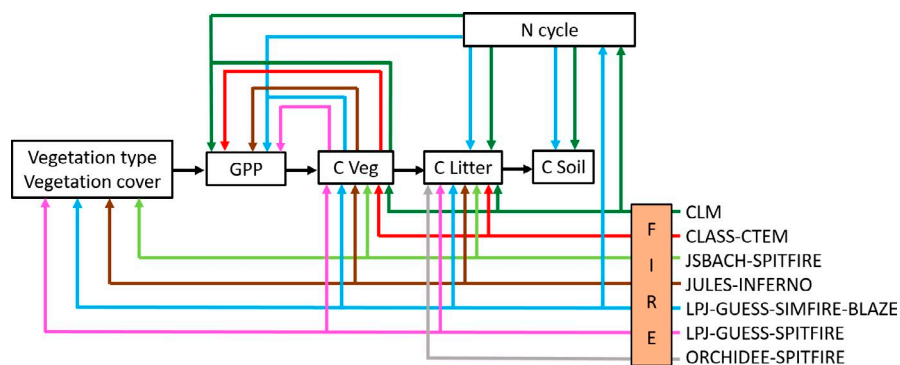
FIGURE 2 Representation of the impact of fire on different components of the carbon/nutrient cycle in the FireMIP models. Note that INFERNNO does not have explicit litter pools but uses two of four soil pools instead. C Litter, carbon stored in litter; C Soil, carbon stored in soil; C Veg: carbon stored in vegetation; CLM, Community Land Model; GPP, gross primary production; LAI, leaf area index; NPP, net primary production; N cycle, nitrogen cycle
