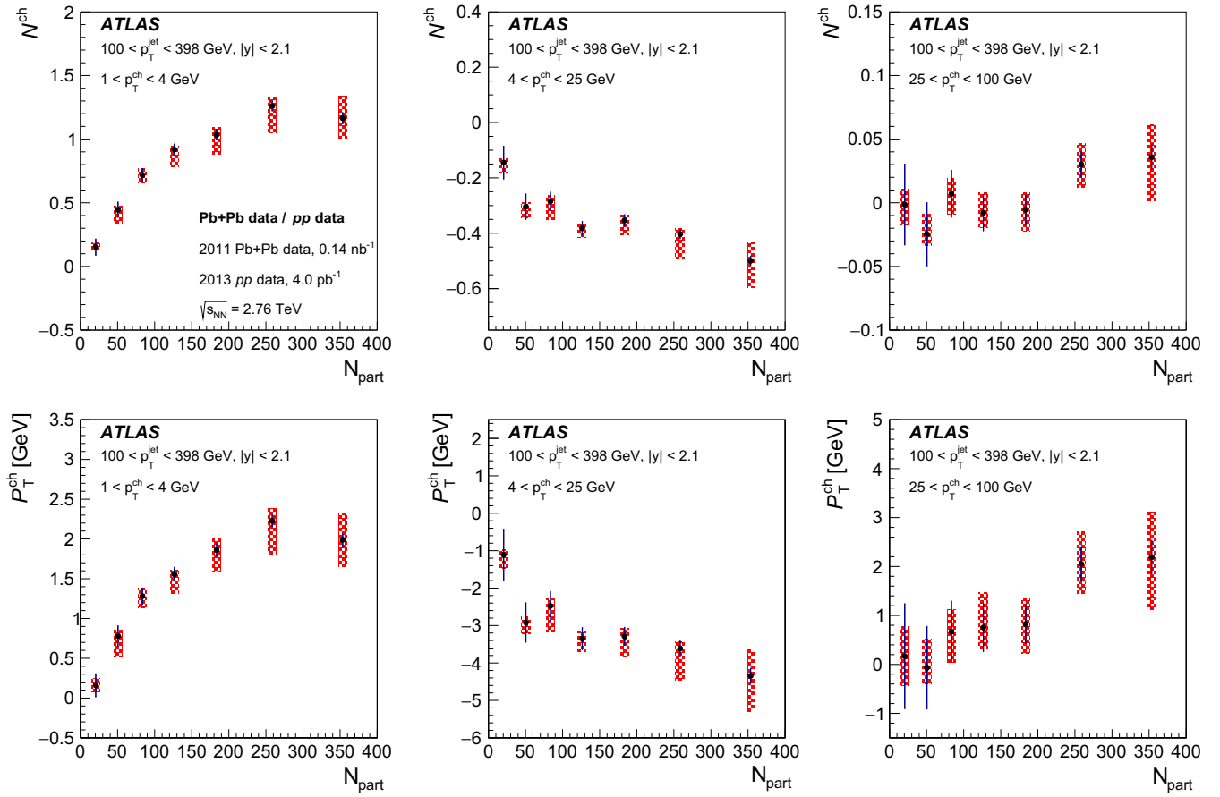
Fig. 8 (Upper panels) The difference N^{\text{ch}} between the total yield of particles in a given p_{\text{T}}^{\text{ch}} interval (indicated in the legend) measured in Pb+Pb collisions and the total yield of particles in the same p_{\text{T}}^{\text{ch}} interval measured in pp collisions. (Lower panels) The difference P_{\text{T}}^{\text{ch}} between the total transverse momentum of particles in a given p_{\text{T}}^{\text{ch}} interval mea-
