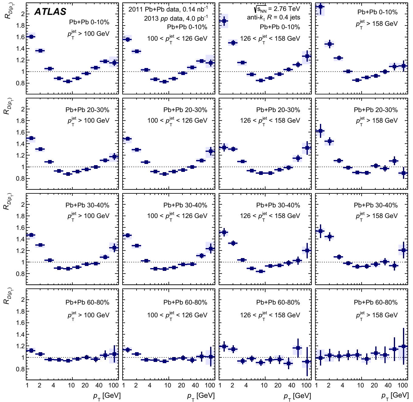
Fig. 6 The ratio R_{D(p_T)} of unfolded D(p_T) distributions measured in heavy-ion collisions to unfolded D(p_T) distributions measured in pp collisions. The R_{D(p_T)} distributions were evaluated in four different centrality bins (rows) and four different selections in jet p_T of jets
