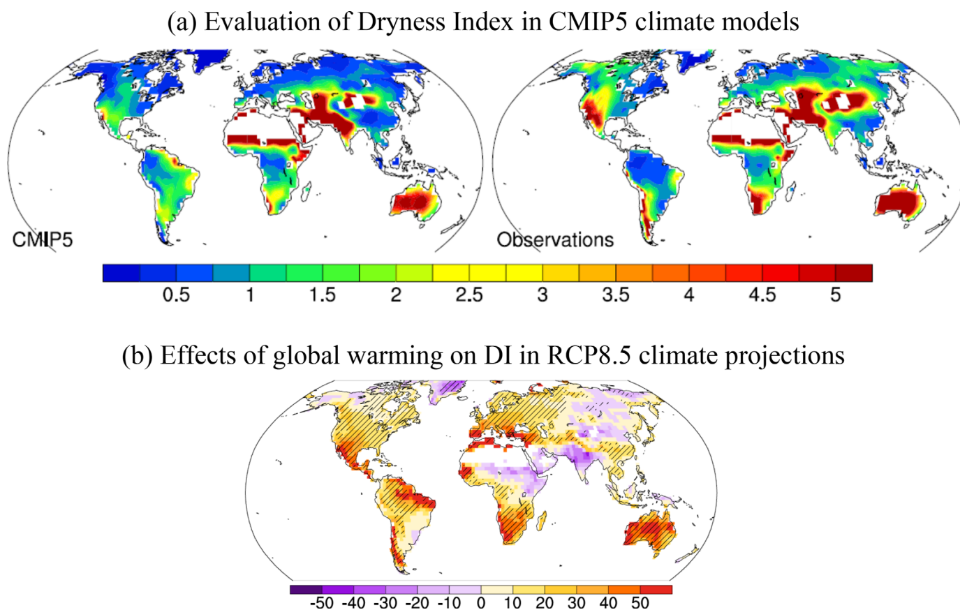
Figure 5. (a) Evaluation of the dryness index in CMIP5 models. Observations show average of three global data sets mentioned in the main text for present climate conditions (1976–2005); (b) projection of DI at the end of 21st century in RCP8.5 climate scenario, shown as the percentage difference from the historical period, i.e., (2081–2100) to (1981–200), hatching shows statistically significant differences at 5% significance level.
