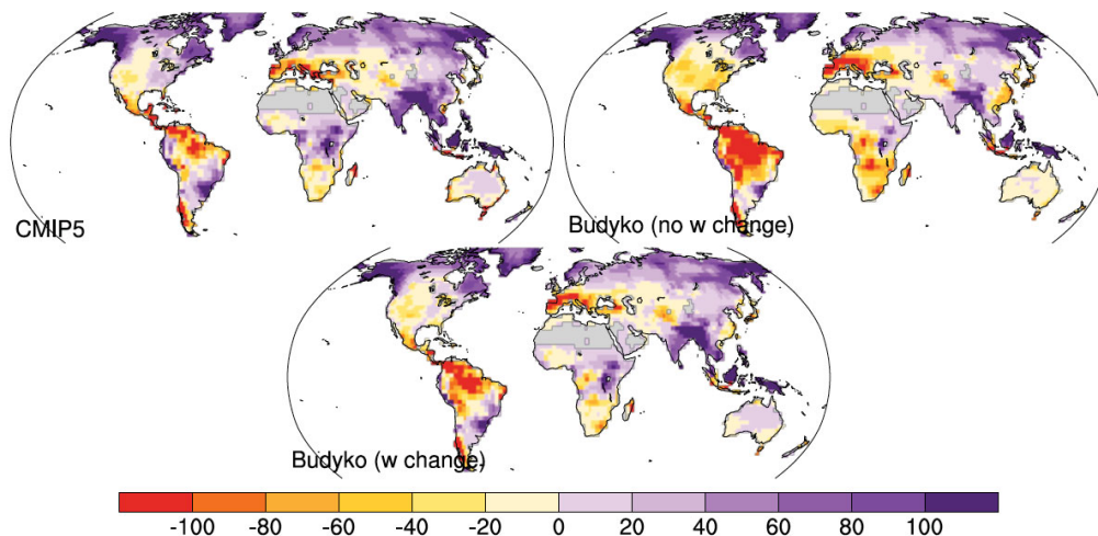
Figure 9. (a) Global runoff change projections in 19 CMIP5 climate models, and using the Budyko framework with and without change in w . Runoff change projections for the RCP8.5 climate scenario are shown as the difference between last and first 20 years, i.e., (2081–2100) to (2006–2025). (b) Spatial distribution of multimodel mean runoff change projections.
