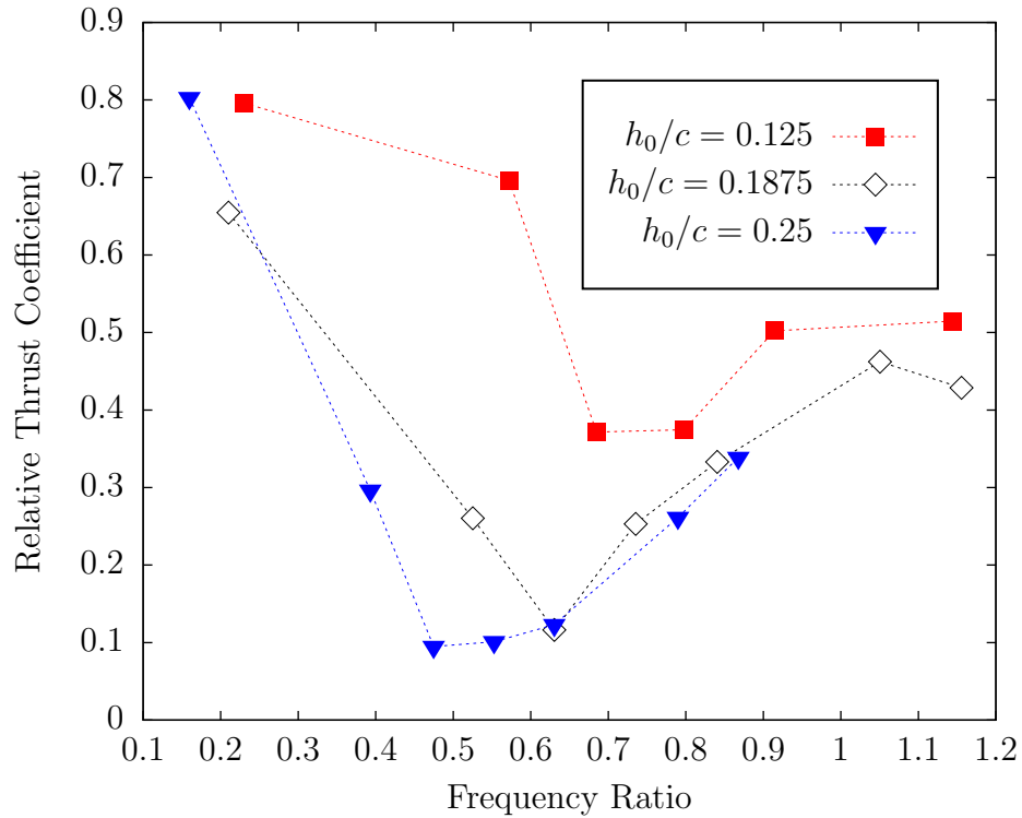
Figure 4.22: Variation with respect to frequency ratio in the relative difference between the thrust coefficients of the foils A3 and B2 at three different heave amplitudes.
