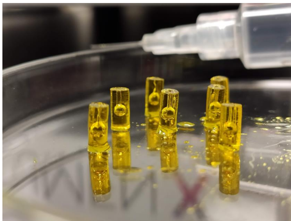
Figure 5. One set of printed spinal cords after printing and removal of uncured material. aCSF is added at this stage post printing to create the organ mimic.
