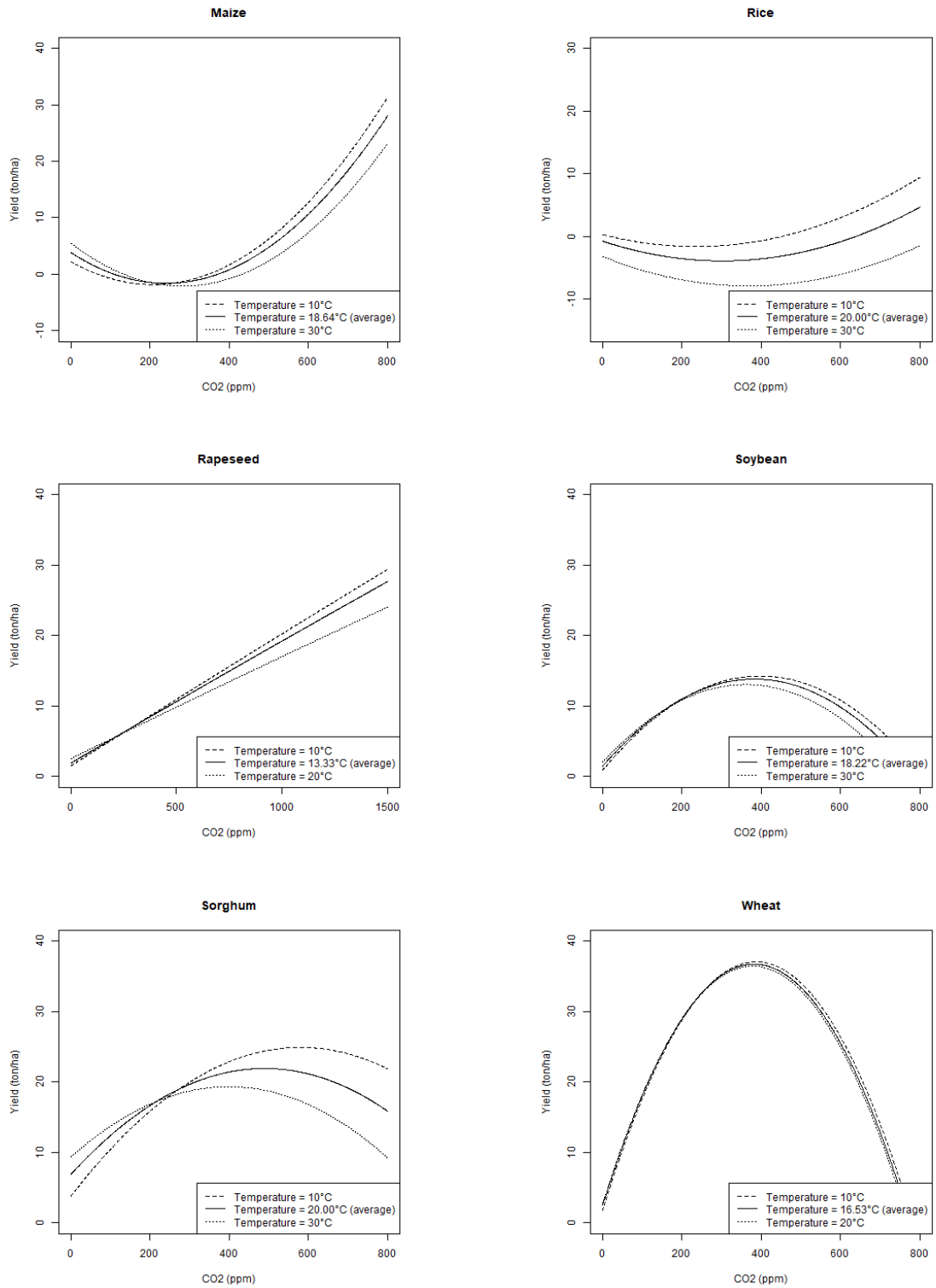
Figure 2.4: CO 2 fertilization Effects on Crop Yields at Different Temperature
