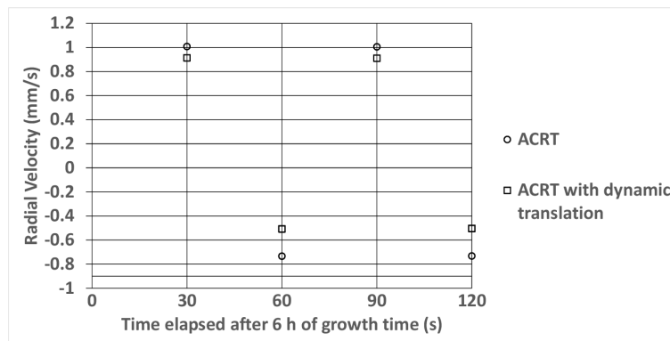
Figure 2. Maximum outward and inward radial velocities in the vicinity of the growth interface after 6 h of growth time.
