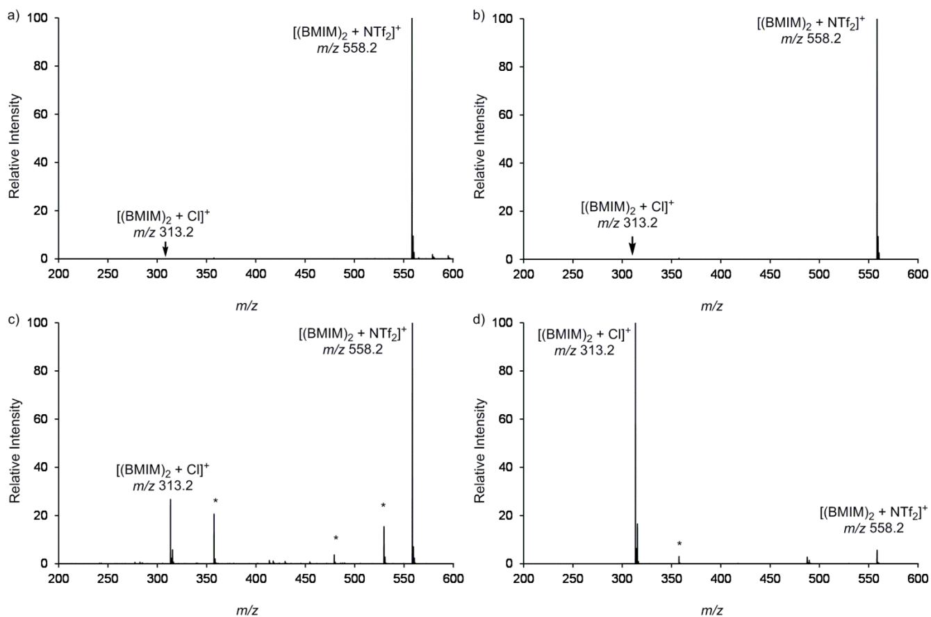
Figure 1: Positive ion ESI mass spectrum of a 1:1 mixture of [BMIM]Cl and [BMIM][NTf 2 ], showing the relative intensities of [(BMIM) 2 + Cl] + ( m/z 313) vs [(BMIM) 2 + [NTf 2 ]] + ( m/z 558) in a) 1:1 H 2 O:MeCN, b) MeOH, c) MeCN, d) CH 2 Cl 2 . Note: Peaks marked with a * are non-aggregate contaminants.
