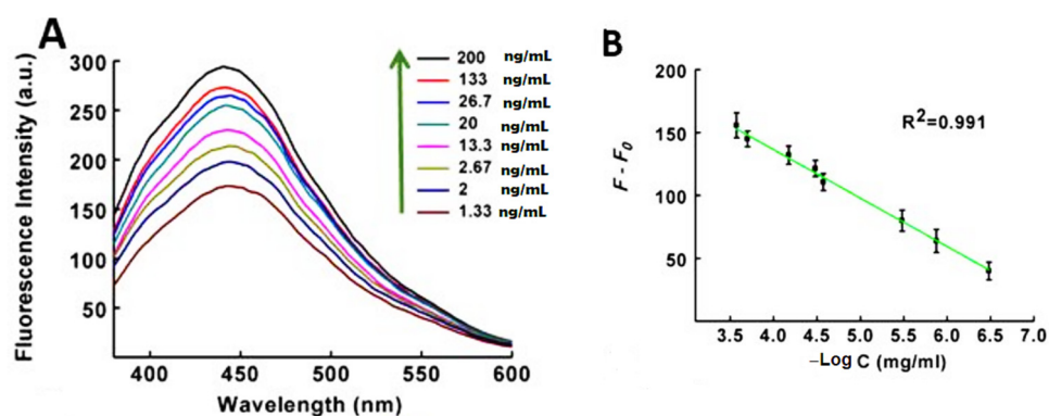
Figure 11. (A) Fluorescence spectra of the assaying model in the presence of varying concentrations of MUC1. (B) The linear relationships between F-F_0 and the concentrations of MUC1. Reprinted with permission from ref. [174]. Copyright 2018, Elsevier.
