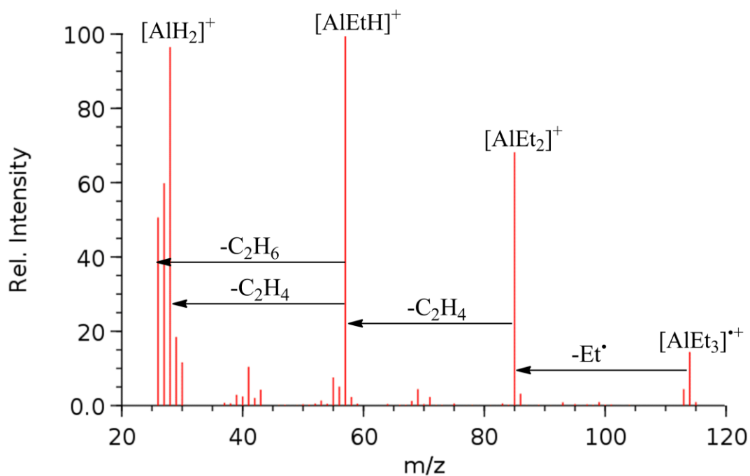
Figure 2. EI mass spectrum of \text{AlEt}_3 (MS data from the NIST Chemistry WebBook). Reproduced with permission from NIST.
