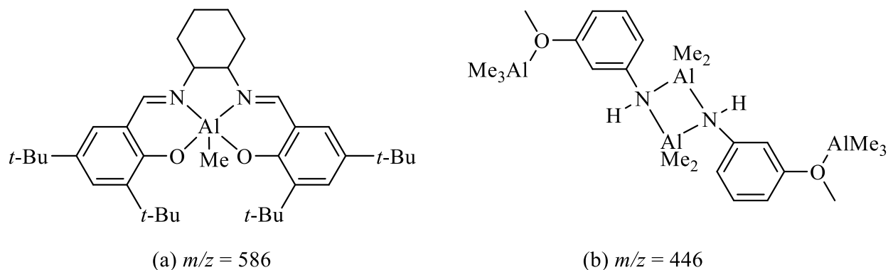
Figure 12. (a) Aluminum salen complex analyzed by ESI, APCI and APPI [M]^+ , 53 (b) [M + H - AlMe_2]^+ . 55 Reproduced with permission from ©John Wiley & Sons Publishing and ©RSC Publishing.
