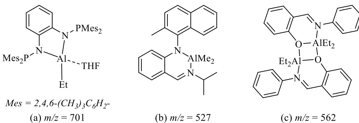
Figure 8. Representative examples of organoaluminum compounds characterized by FAB. Highest mass ion observed was (a) [M-THF] ++ , 34 (b) [M+Na] + , 36 (c) [M] ++ . 37 Reproduced with permission from
