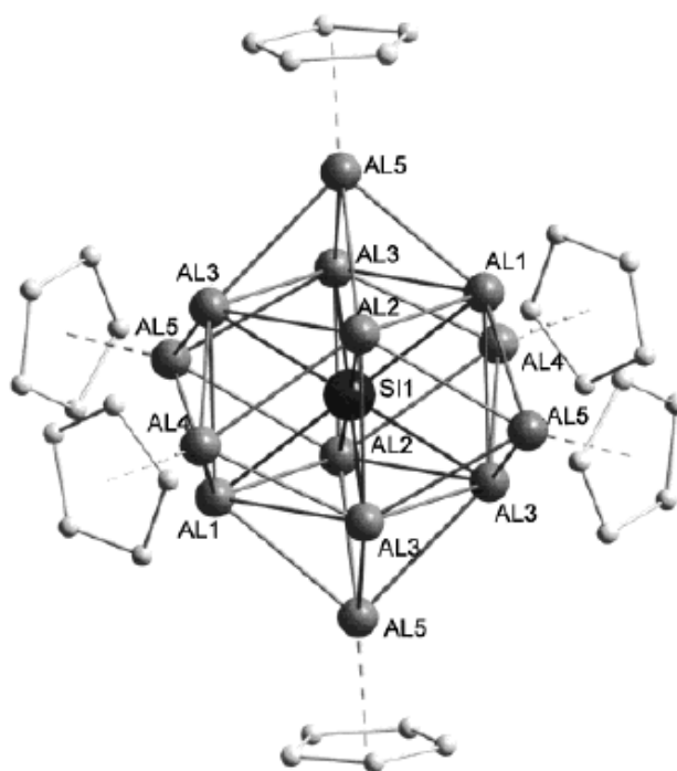
Figure 13. X-ray structure of a Cp*Al-Si cluster (methyl groups omitted for clarity) analyzed by MALDI-TOF MS - m/z 1217 ( M^+ ), 1081 ( M^+ - Cp^* ). 59 Reproduced with permission from ©ACS Publishing.
