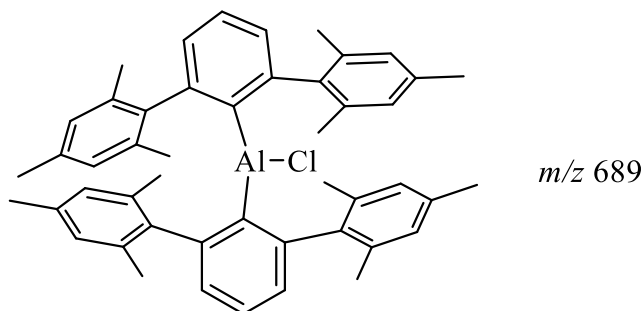
Figure 14. An organoaluminum compound characterized by DART as an [M + H]^+ ion. 61 Reproduced with permission by ©Wiley-VCH Verlag.
