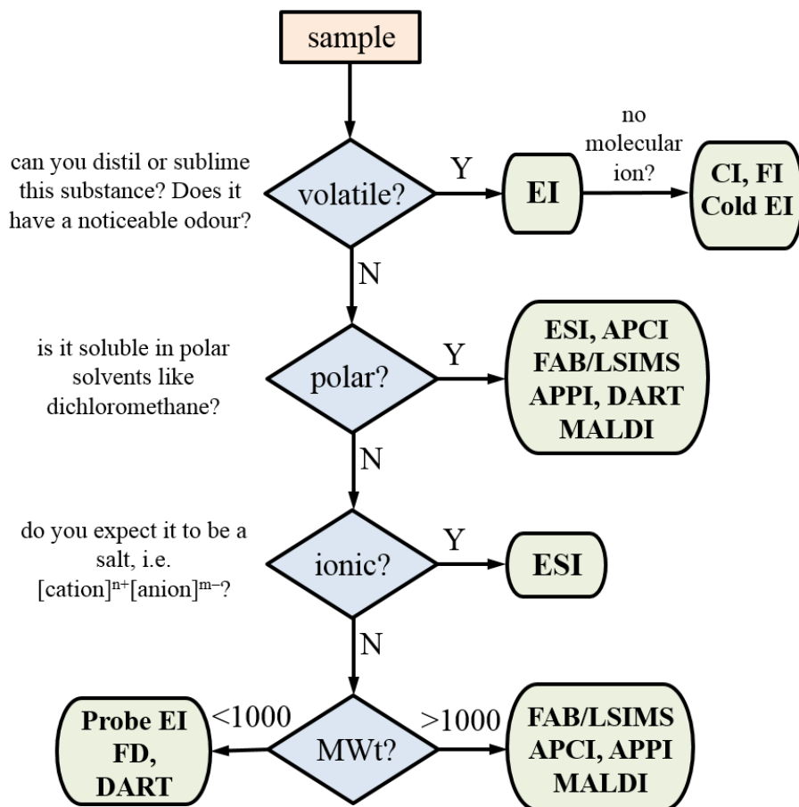
Figure 15. How to choose an ionization technique - a rough guide.
