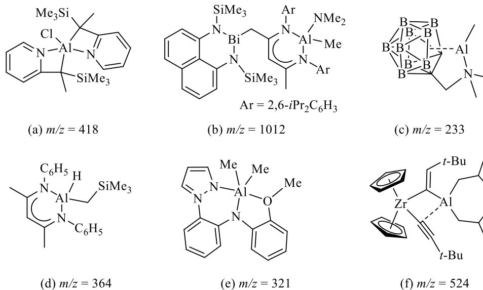
Figure 5. Structures and m/z values of some organoaluminums characterized by EI MS. The molecular ion was observed for each compound (a), 10 (b), 11 (c), 12 (d), 13 (e), 14 and (f). 15 Reproduced with permission from
