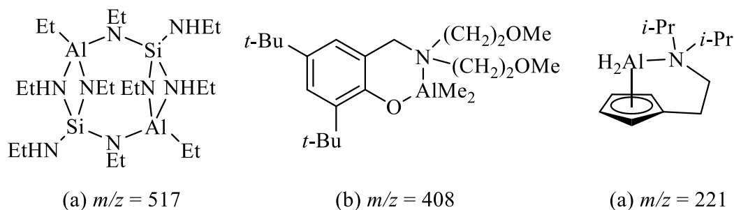
Figure 6. Structures and m/z values of some CI MS-characterized organoaluminums. (a) isobutane reagent gas [M+H]^+ ; 23 (b) [M+H]^+ ; 21 (c) CH_4 reagent gas [M+H]^+ . 24 Reproduced with permission from ©RSC Publishing, ©ACS Publishing and ©Wiley-VCH Verlag.
