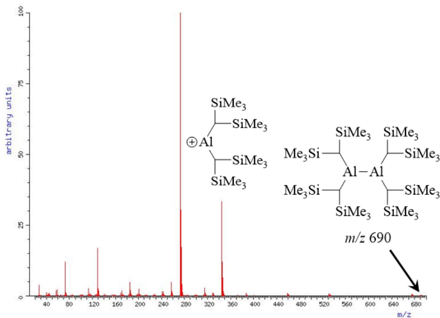
Figure 4. EI-MS of (\text{Al}(\text{CH}(\text{SiMe}_3)_2)_2)_2 . 9 Spectral data were obtained from Wiley Subscription Services, Inc. (US). Note the low abundance of the molecular ion, typical of the EI-MS of high molecular weight analytes. Reproduced by permission of ©DeGruyter Publishing.
