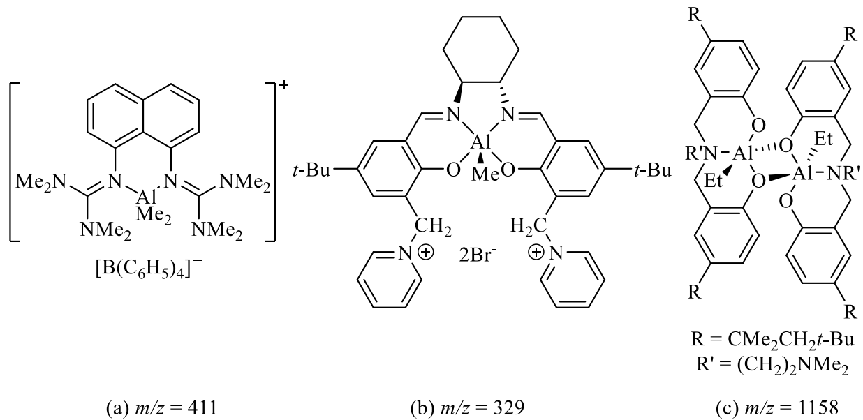
Figure 9. Structures of some organoaluminum compounds characterized by ESI-MS (a) [M]^+ , 43 (b) [M-2Br]^{2+44} (c) [M+H]^+ . 45 Reproduced with permission from ©Wiley-VCH Verlag, and ©RSC Publishing.
