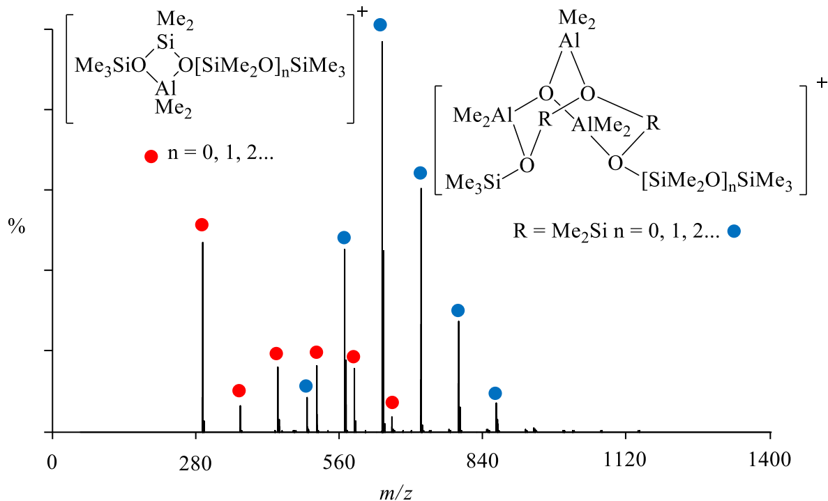
Figure 10. Positive ion ESI MS of a mixture of methylaluminoxane (MAO) and trace levels of silicone grease in fluorobenzene solution with proposed structures of the major ions depicted. Reproduced with permission from ©ACS Publishing.
