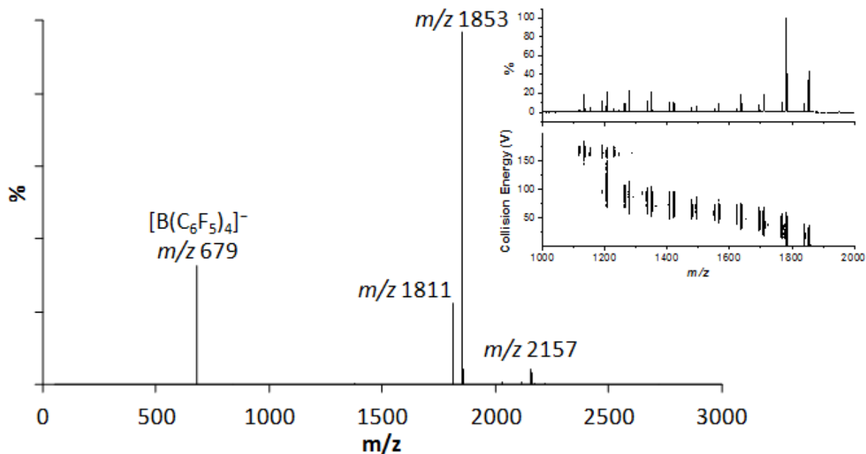
Figure 11. Corresponding negative ion spectrum of MAO + silicone grease in the presence of [(^{13}C_{18}H_{37})_4N][B(C_6F_5)_4]^- standard; inset - Tandem MS/MS spectrum and energy dependent (ED) ESI MS of the anion with m/z 1853 showing 10 consecutive losses of AlMe_3 as the collision energy is increased.
