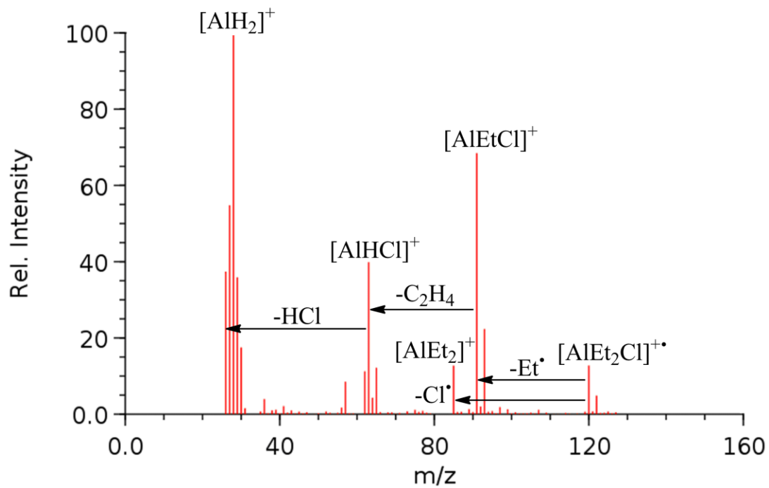
Figure 3. EI mass spectrum of AlEt 2 Cl (MS data from the NIST Chemistry WebBook). Reproduced with permission from NIST.
