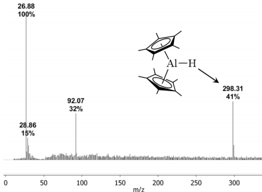
Figure 7. LIFDI-MS of (C_5Me_5)_2AlH from a toluene solution. Reproduced with permission from ©RSC Publishing.
