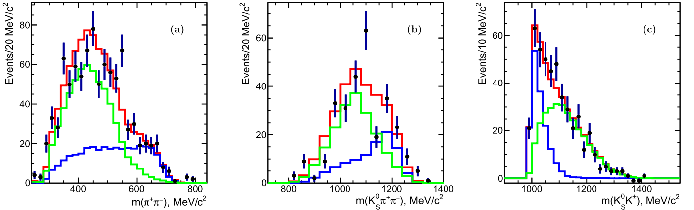
Fig. 7. The experimental m(\pi^+ \pi^-) (a), m(K_S^0 \pi^+ \pi^-) (b), and m(K_S^0 K^\pm) (c) invariant mass distributions in comparison with the simulation (red histogram). The blue and green histograms are the MC simulation contributions from the e^+e^- \rightarrow f_1(1285)\rho and e^+e^- \rightarrow f_1(1420, 1510)\rho reactions, respectively.
