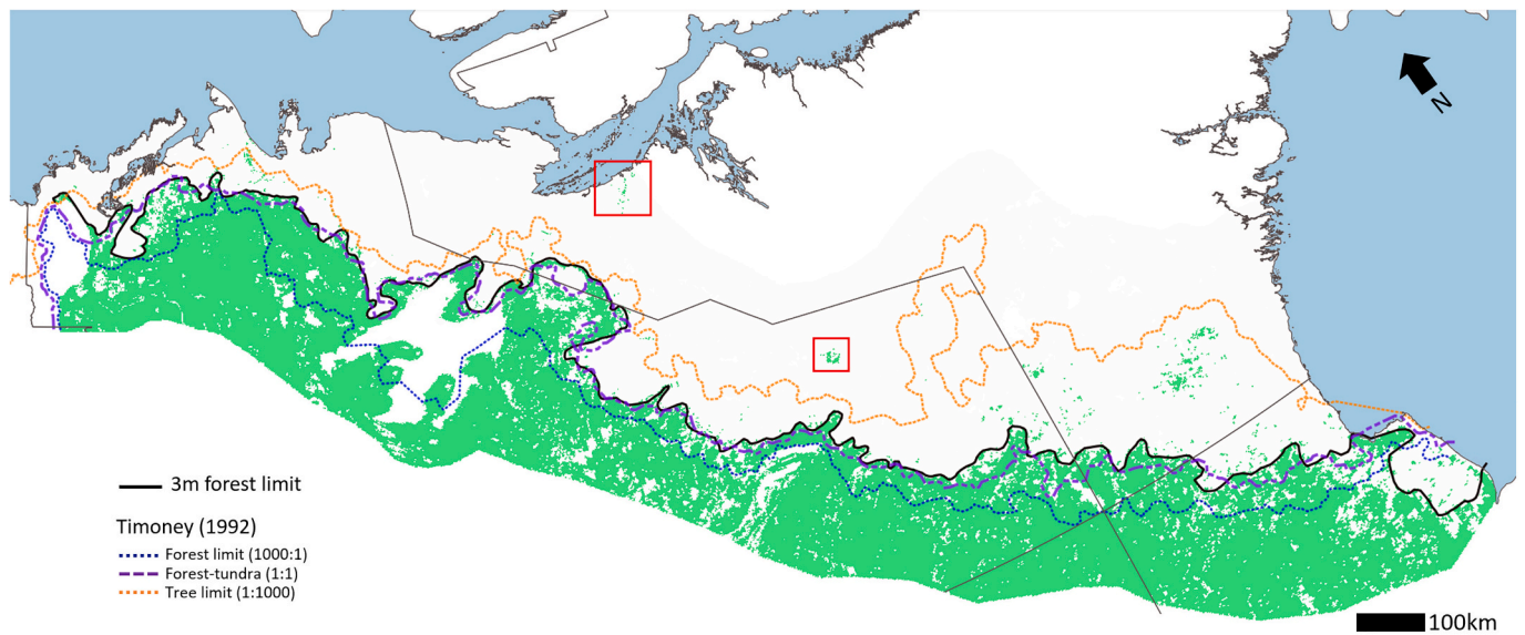
Fig. 7. Map of 3 m canopy distribution, green colour indicates average height of at least 3 m in a 1 km grid cell. The black line delineates the northern extent of continuous forest (the southern extent of continuous forest extends beyond the study area). The dashed lines show the forest limit, forest-tundra and tree limits mapped by Timoney et al. (1992) . Red boxes show non-spatially congruous regions above the tree limit that were examined using high-resolution (<1 m spatial resolution) WorldView-2 imagery. (For interpretation of the references to colour in this figure legend, the reader is referred to the web version of this article.)
