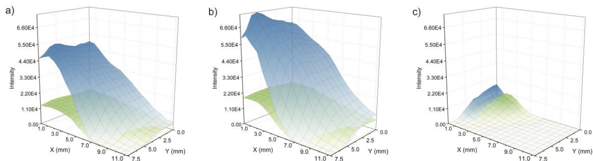
Figure 8. PPN and TMA Ion Intensity at 26 \mu\text{M} in MeCN with a) 200 \text{L}\cdot\text{hr}^{-1} desolvation gas flow rate, b) 50 \text{L}\cdot\text{hr}^{-1} and c) 25 \text{L}\cdot\text{hr}^{-1} . Refer to table S1, experiments 4, 6 and 8, in supporting information for experiment parameters.
