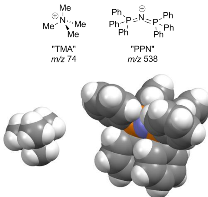
Figure 1. The two cations investigated in this study. Space-filling models were generated from published crystallographic data files. [12]
