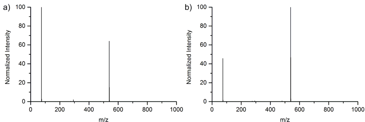
Figure 3. Mass spectra of 0.0260 mM PPN ( m/z 538.2) and TMA ( m/z 74.1) in acetonitrile for capillary positions (a) far and (b) near the mass spectrometer aperture
