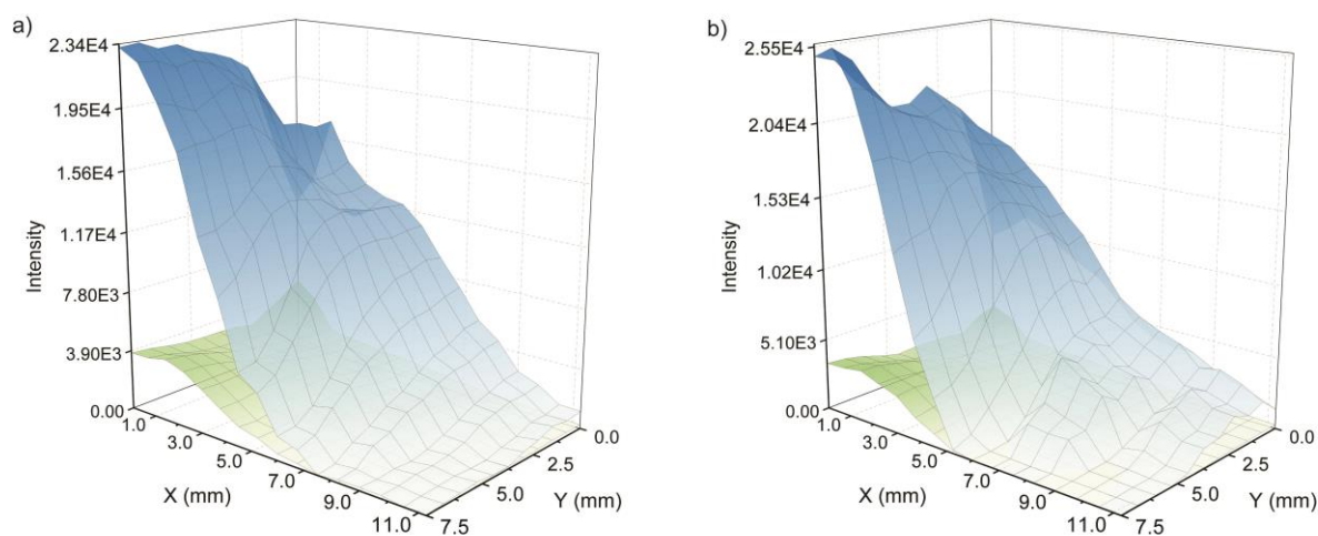
Figure 7. PPN (above) and TMA (below) Ion Intensity at 0.260 mM in MeCN with a) 50 L·hr -1 cone gas flow rate and b) 100 L·hr -1 . Refer to table S1, experiments 2 and 3, in supporting information for experiment parameters.
