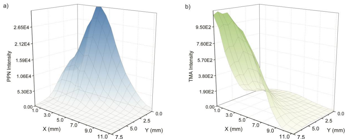
Figure 6. Intensity vs. capillary position for a) PPN vs. b) TMA in water. Note the orders-of-magnitude difference in the vertical axes in the two plots. Refer to table S1, experiment 11, in supporting information for experiment parameters.
