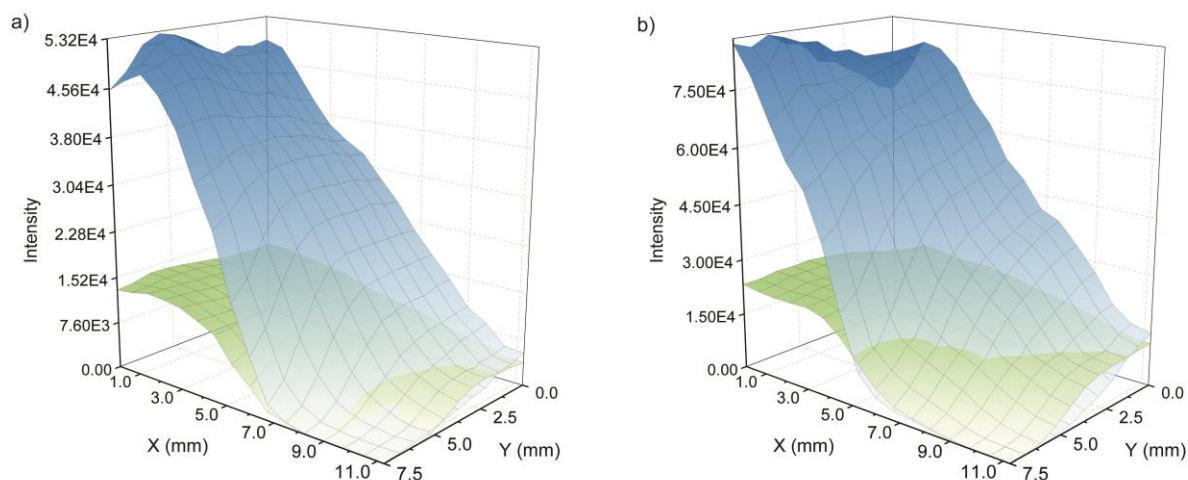
Figure 10. PPN and TMA ion intensity at 26 \mu\text{M} in MeCN with a desolvation temperature of a) 189°C and b) 89°C. Refer to table S1, experiments 4, 10, and 13, in supporting information for experiment parameters.
