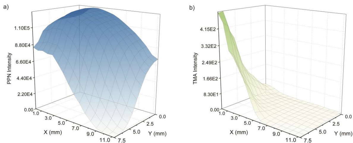
Figure 5. Intensity vs. capillary position for a) PPN vs. b) TMA in methanol. Note the difference in the vertical axes in the two plots (0–150,000 vs. 0–500). Refer to table S1, experiment 5, in supporting information for experiment parameters.
