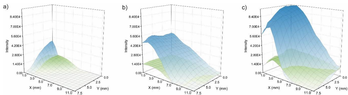
Figure 9. PPN and TMA ion intensity at 26 uM in MeCN with a source temperature of a) 39°C, b) 89°C, and c) 150°C. Refer to table S1, experiments 4, 10, and 13, in supporting information for experiment parameters.
