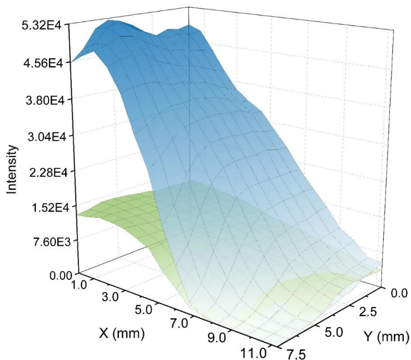
Figure 4. Overlaid ESI-MS intensities of an equimolar mixture of PPN and TMA at varying capillary positions. Note the divergent behaviour far from the MS aperture. Refer to table S1, experiment 4, in supporting information for experiment parameters.
