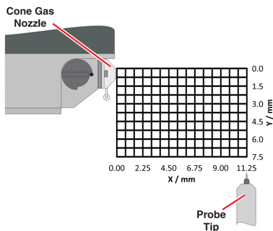
Figure 2. Illustration of the spray head in its most distant position with respect to the aperture. The grid defines the locations of each analysis. A photo of the ESI source with an overlaid grid may be found in the SI (figure S15).
