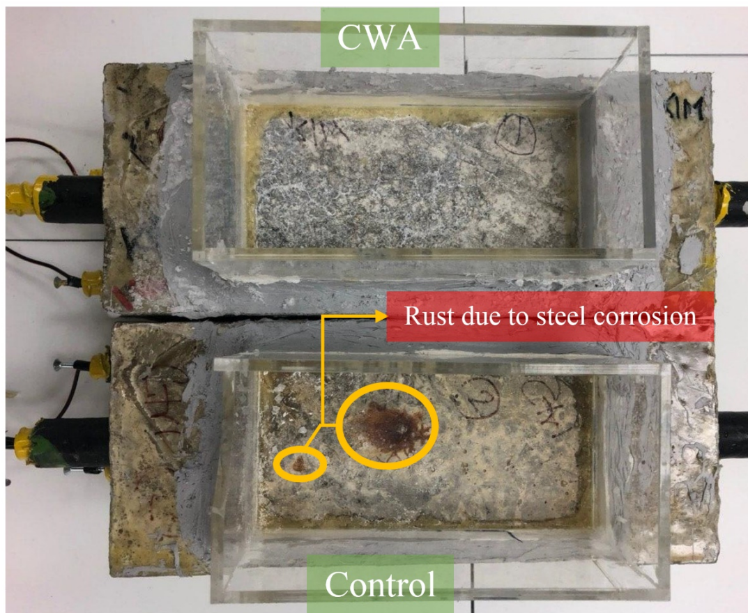
Figure 6. Visual inspection of corrosion in control and CWA-modified concrete beams.
