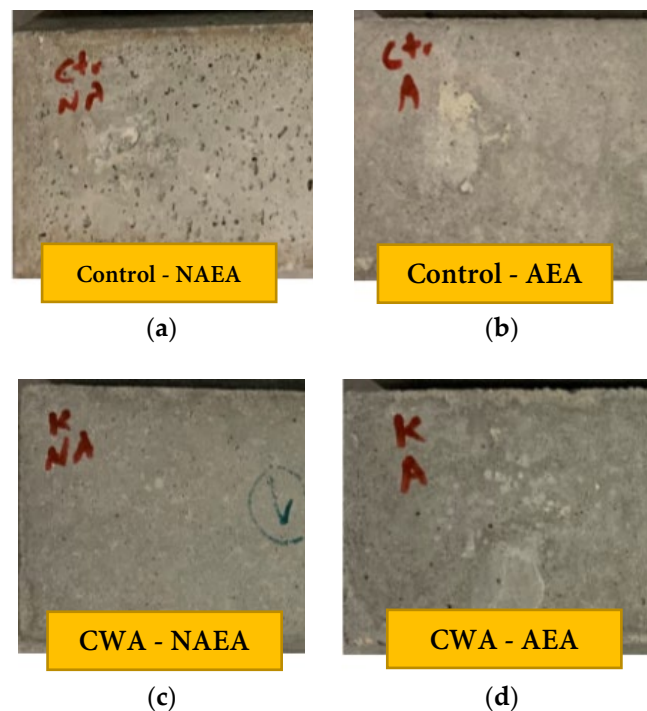
Figure 11. Surface of concrete samples exposed to 300 freeze/thaw cycles: (a) Control—NAEA; (b) Control—AEA; (c) CWA—NAEA; (d) CWA—AEA.
