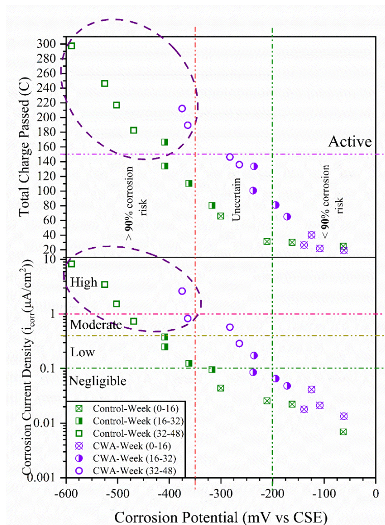
Figure 10. Relationship between corrosion potential, total charge passed and current density.
