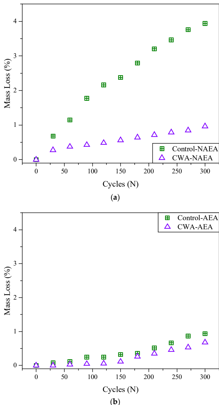
Figure 13. Percentage of mass loss of (a) non-air-entrained and (b) air-entrained concrete samples.
