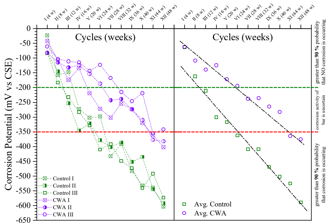
Figure 7. Half-cell potential measurement results.
