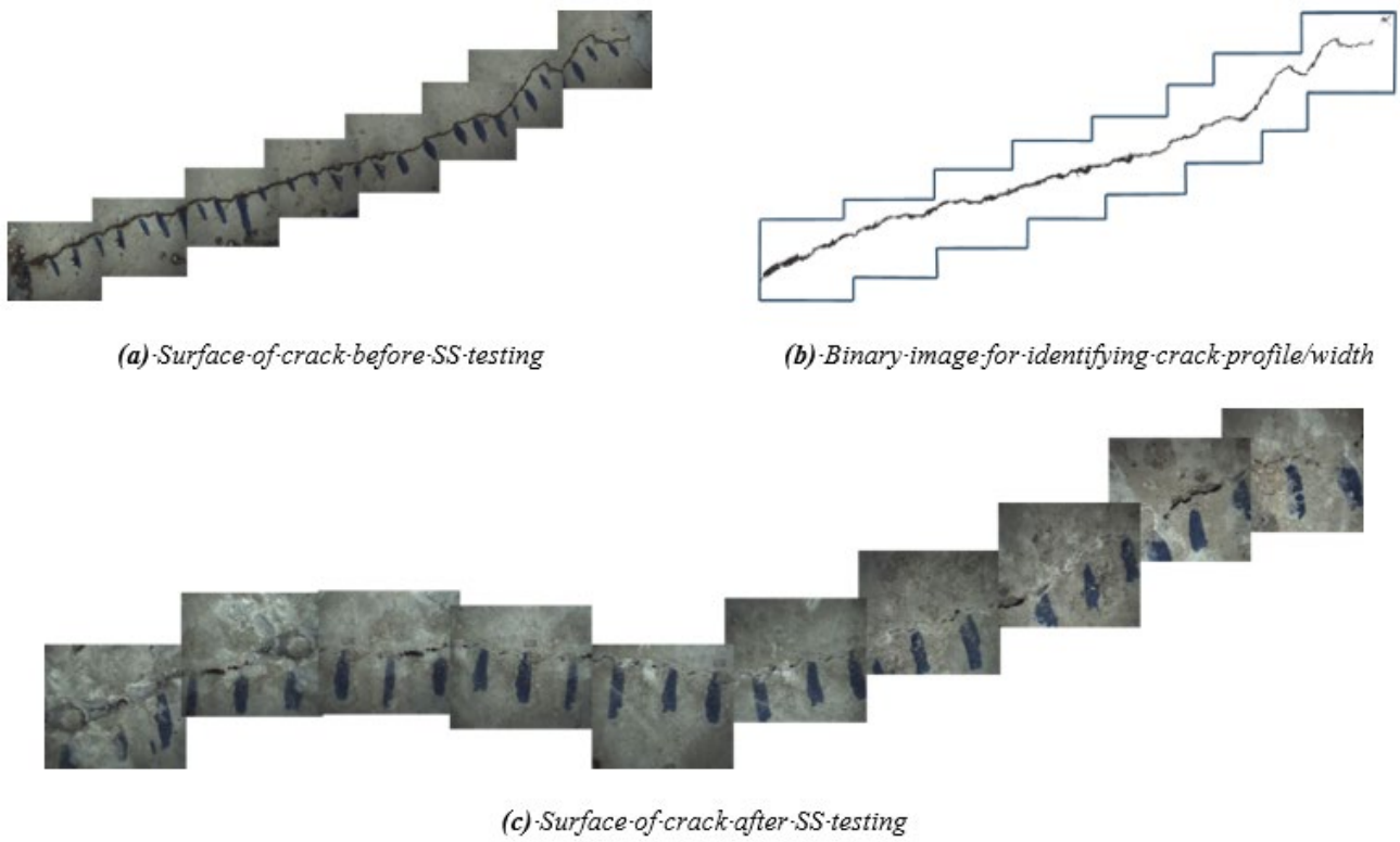
Figure 16. Crack surface of control specimen. (a) Before sealing; (b) binary image of isolated crack; (c) after sealing.
