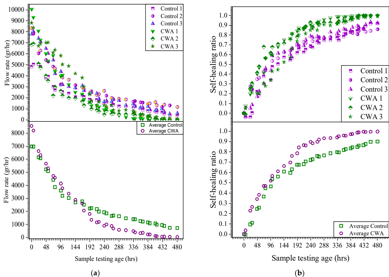
Figure 18. (a) Flow rate vs. time; (b) self-sealing ratio.
