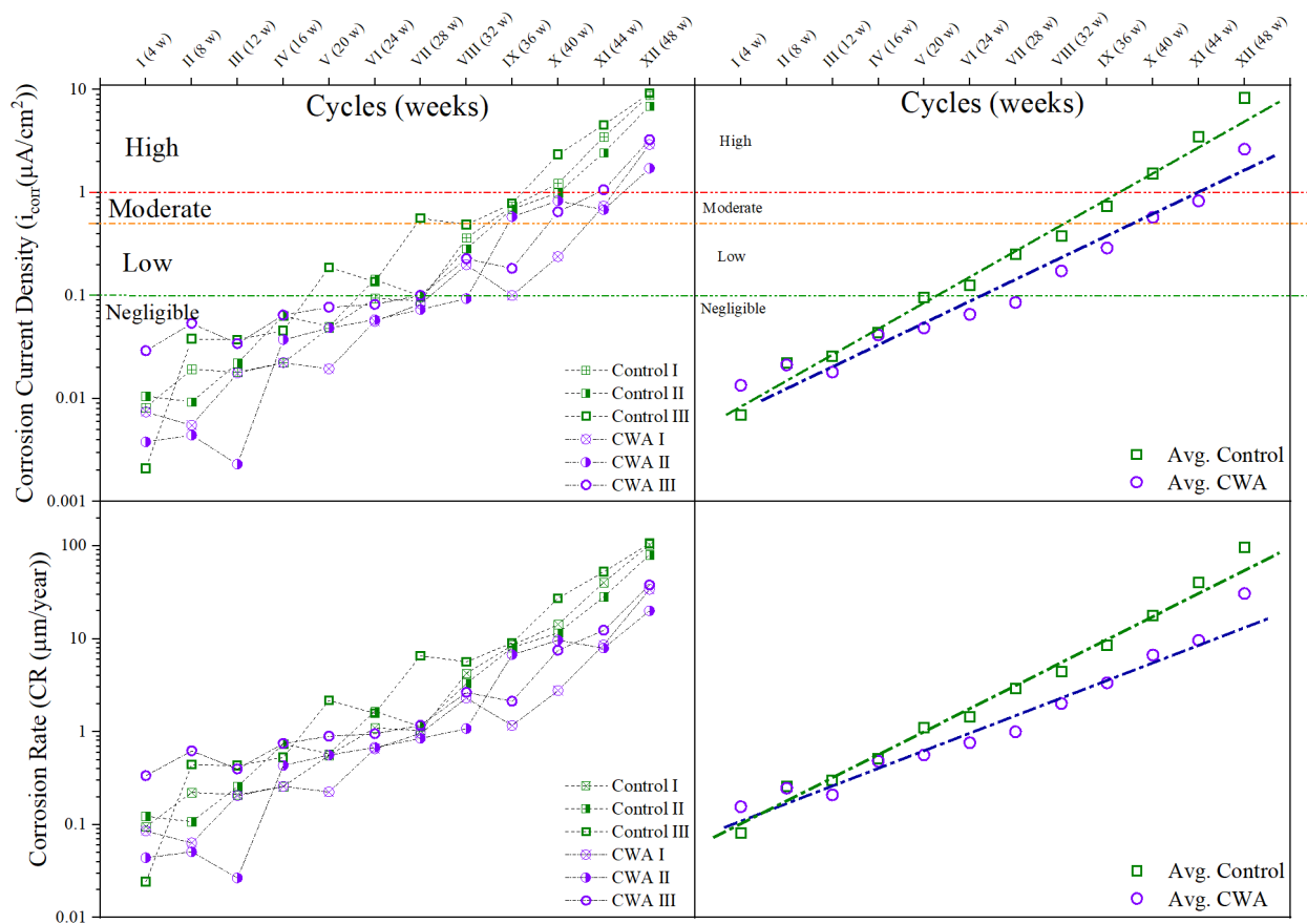
Figure 9. Corrosion current density and rate for reinforced concrete beams exposed to NaCl for 48 weeks.
