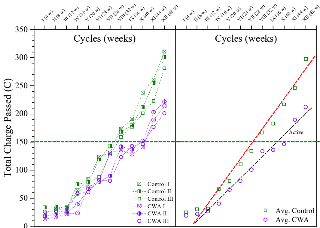
Figure 8. Macro-cell corrosion results.
