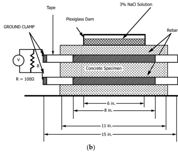
Figure 1. Concrete Beam (All measurements in inches): (a) schematic specimen configuration and cross-section view; (b) side view.
