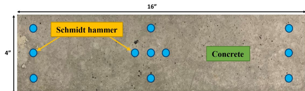
Figure 4. Schematic locations for using a Schmidt hammer.
