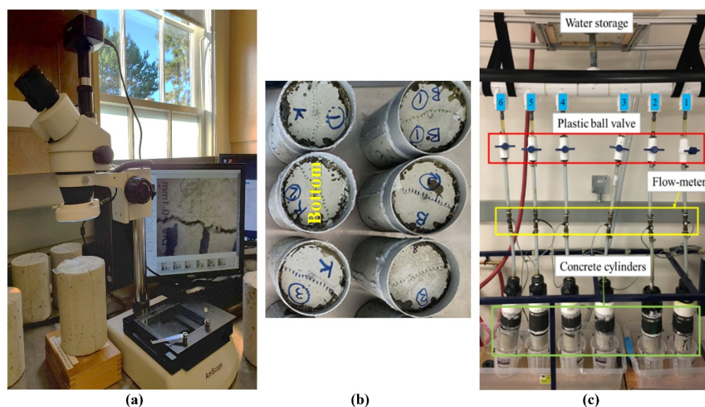
Figure 5. (a) Crack investigation using optical microscope. (b) Cylinders prepared for testing (bottom side exposed to water flowing from tank). (c) Self-sealing setup [58].
