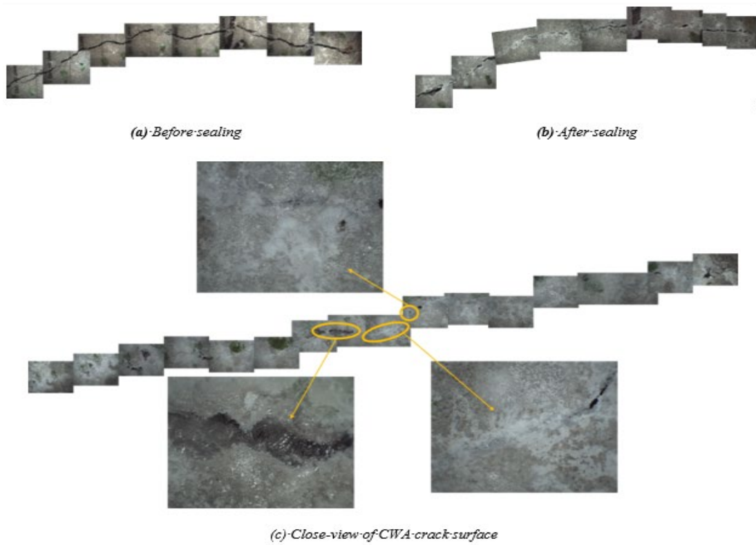
Figure 17. Crack surface of CWA specimen. (a) Before sealing; (b) after sealing; (c) close view of crack surface.
