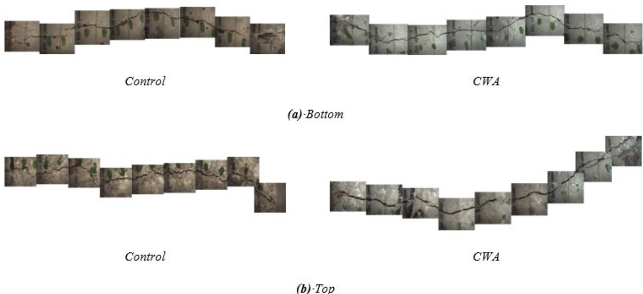
Figure 15. Crack profile of CWA and control concretes (a) Cylinder bottom during casting (b) Cylinder top during casting.
